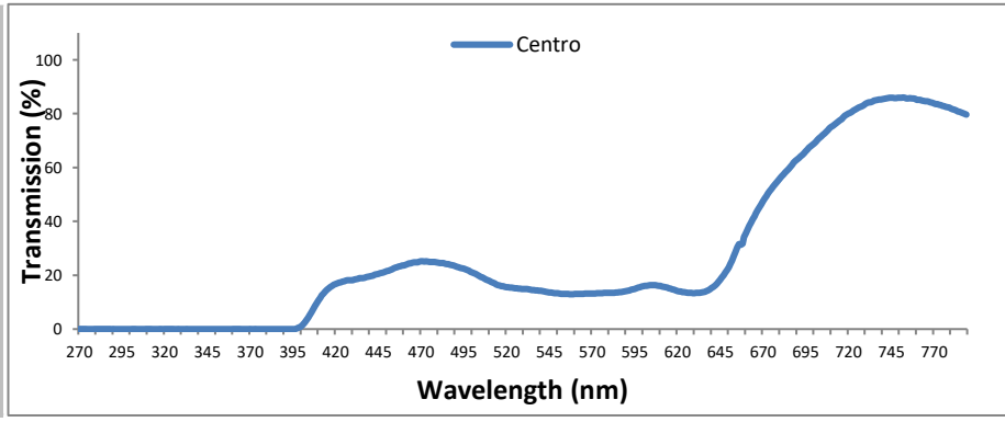
Spectral Transmittance
